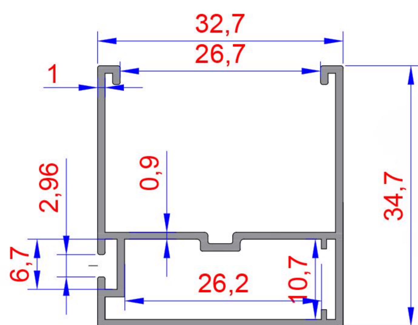
INSECT SCREEN PROFILE
