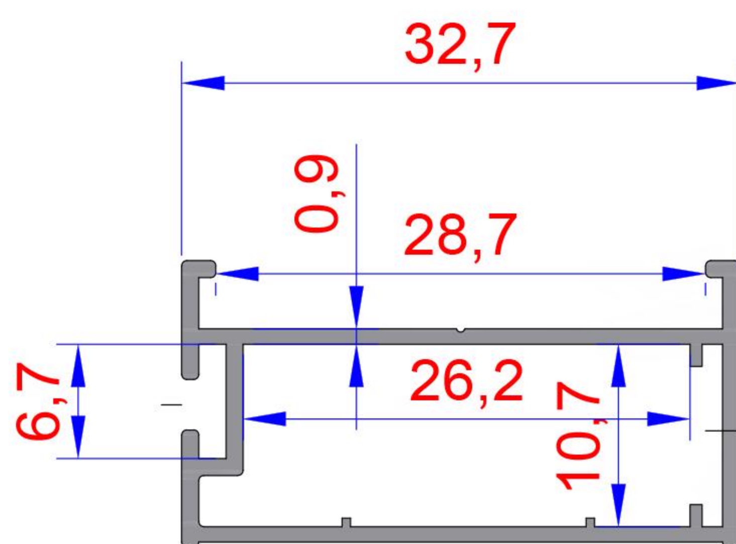
INSECT SCREEN PROFILE
