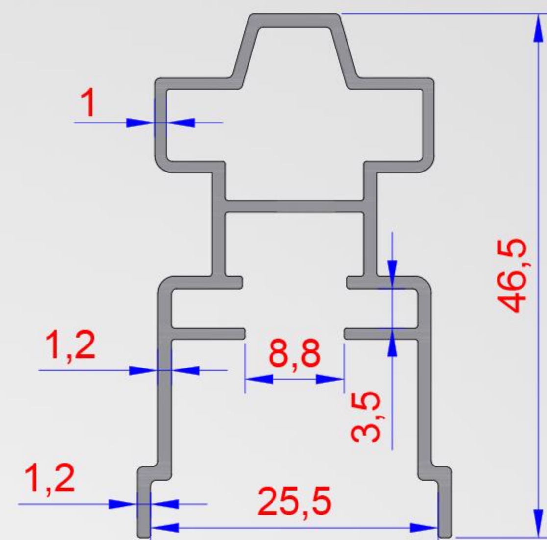
INSECT SCREEN PROFILE
