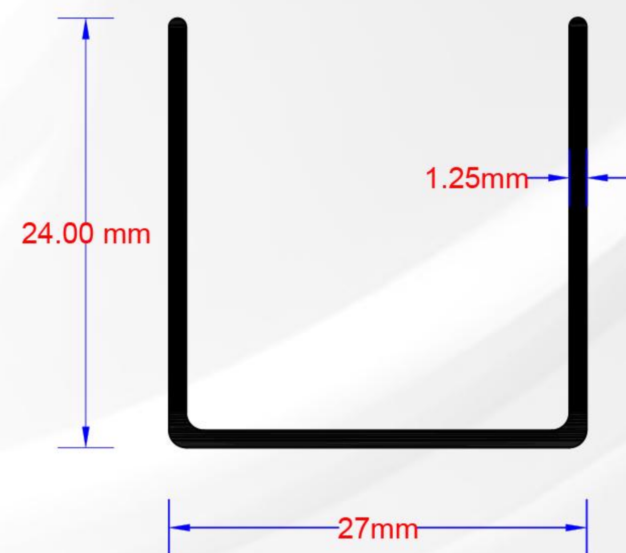
GALVANIZED REINFORCEMENT AK-82105
