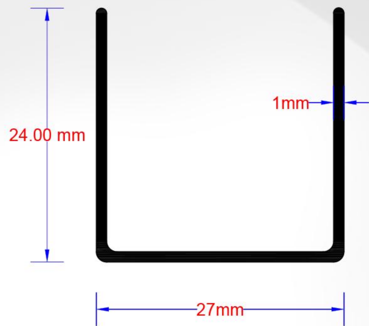
GALVANIZED REINFORCEMENT AK-82104
