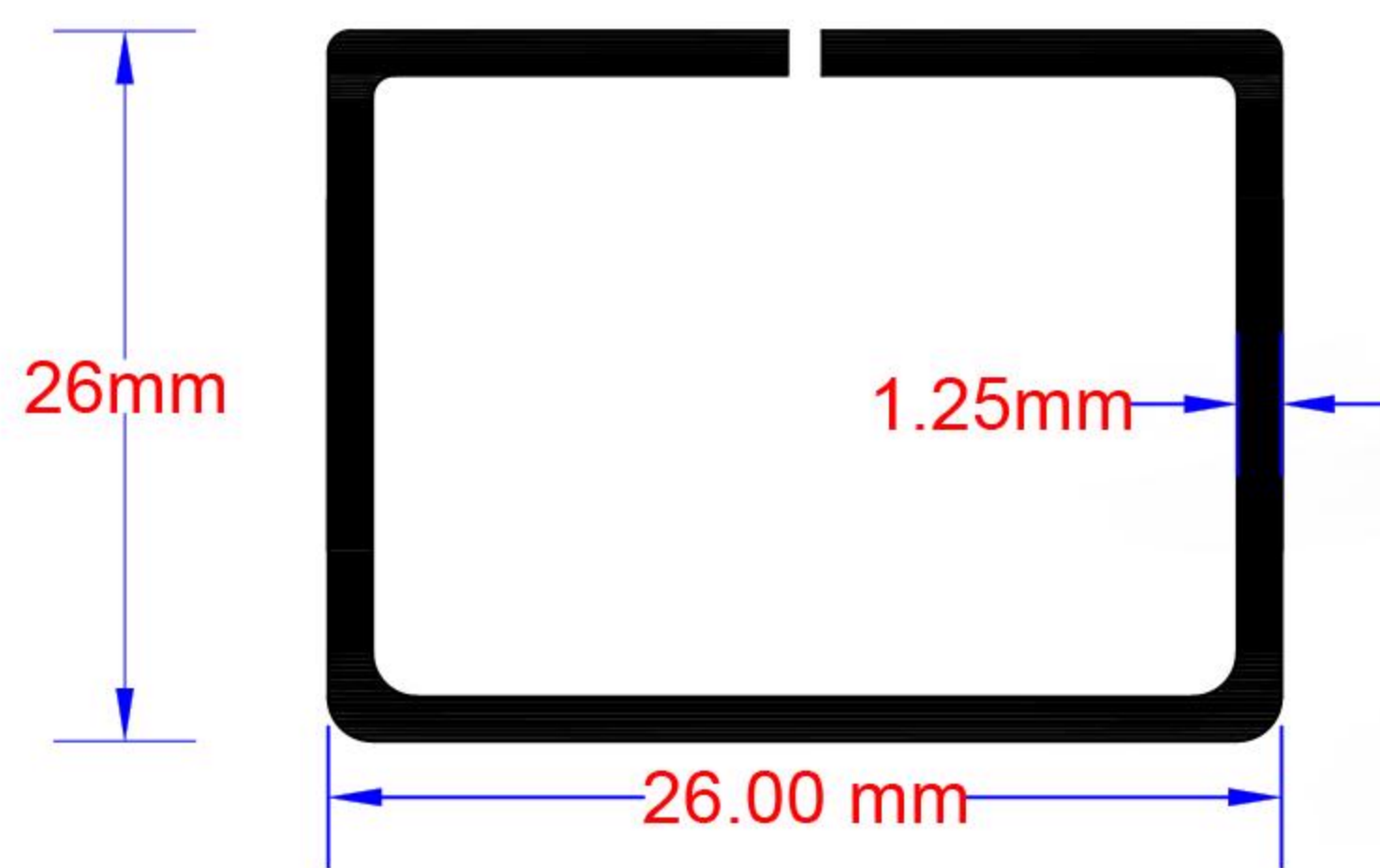
GALVANIZED REINFORCEMENT AK-82106
