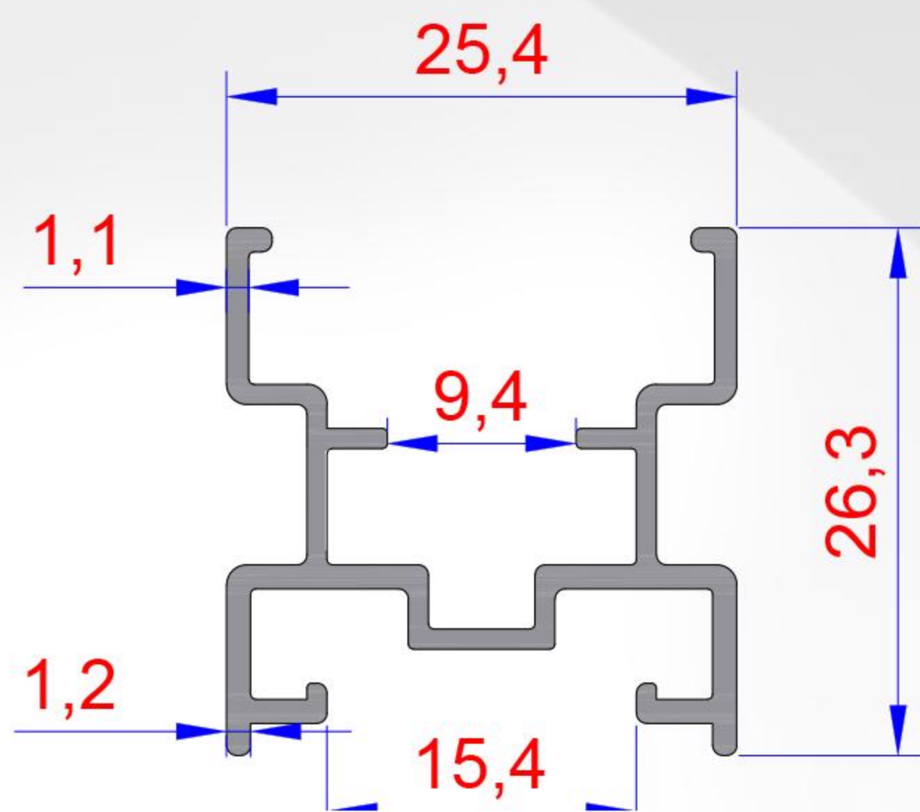
INSECT SCREEN PROFILE
