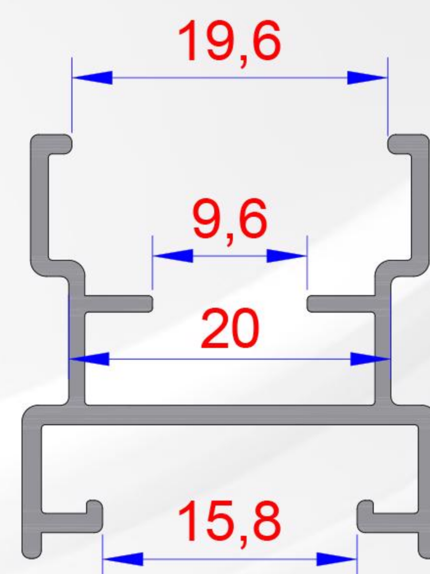
INSECT SCREEN PROFILE
