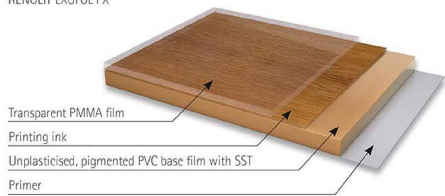
Diagram showing the structure of the exterior film RENOLIT EXOFOL PX
